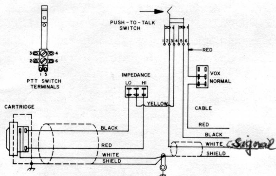
INTERNAL CONNECTIONS FIGURE 2
